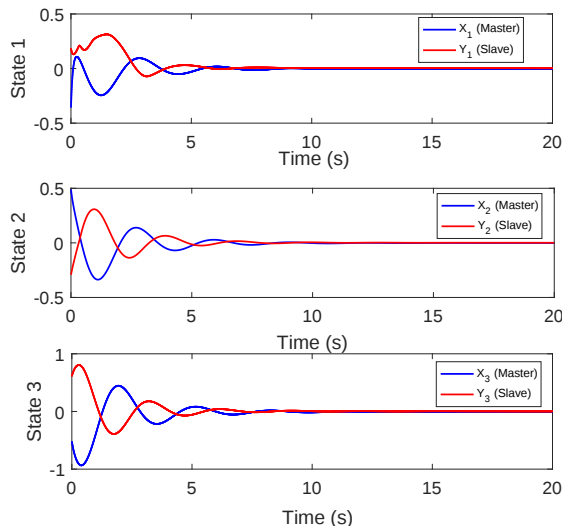
Figure 1. Master and slave state trajectories.
